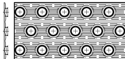
FIN LAYOUT Ø3/8"x0.866" (Ø9.525mm. x 21.996mm) WAVE SLIT SURFACE / STRAIGHT EDGES
