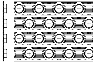
FIN LAYOUT 3/8" (1"x0.75") SLIT/STRAIGHT EDGES
