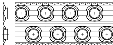
FIN LAYOUT Ø3/8 (1 "X0.866") SINE WAVE RIPPLED EDGES
