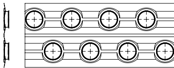
FIN LAYOUT 5/8" (38.1mm.x33mm.) CORRUGATED/RIPPLED EDGES
