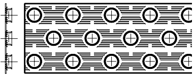
FIN LAYOUT Ø7mm. (21mm. x 12.7mm.) LOUVERED SURFACE / STRAIGHT EDGES
