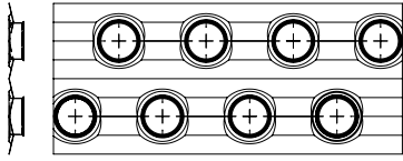
FIN LAYOUT 1/2" (31.75mm.x27.5mm.) CORRUGATED/RIPPLED EDGES
