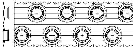
FIN LAYOUT 5/16" (1"x0.75") CORRUGATED/RIPPLED EDGES
