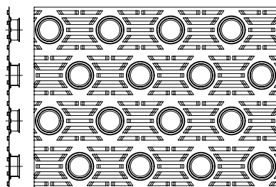
FIN LAYOUT 5/16" (1"x0.75") SLIT/STRAIGHT EDGES
